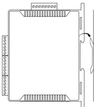
– Installation method of guide rail –
