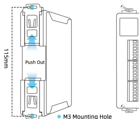
– Screw installation method –
